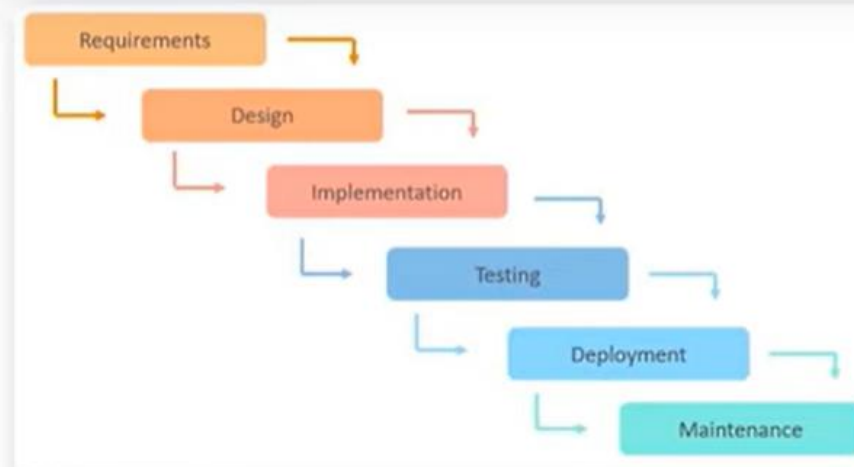
Waterfall Model
